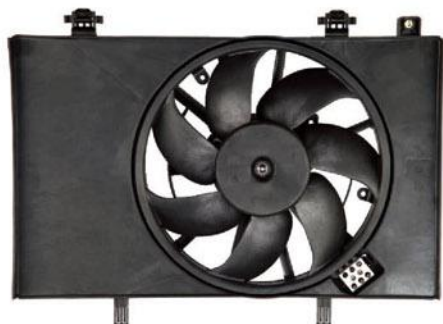
OEM NO :ZJ36-15-025 DC:12V Suitable automotive type: ford fiesta 适用车型: 福特嘉年华 (新)
