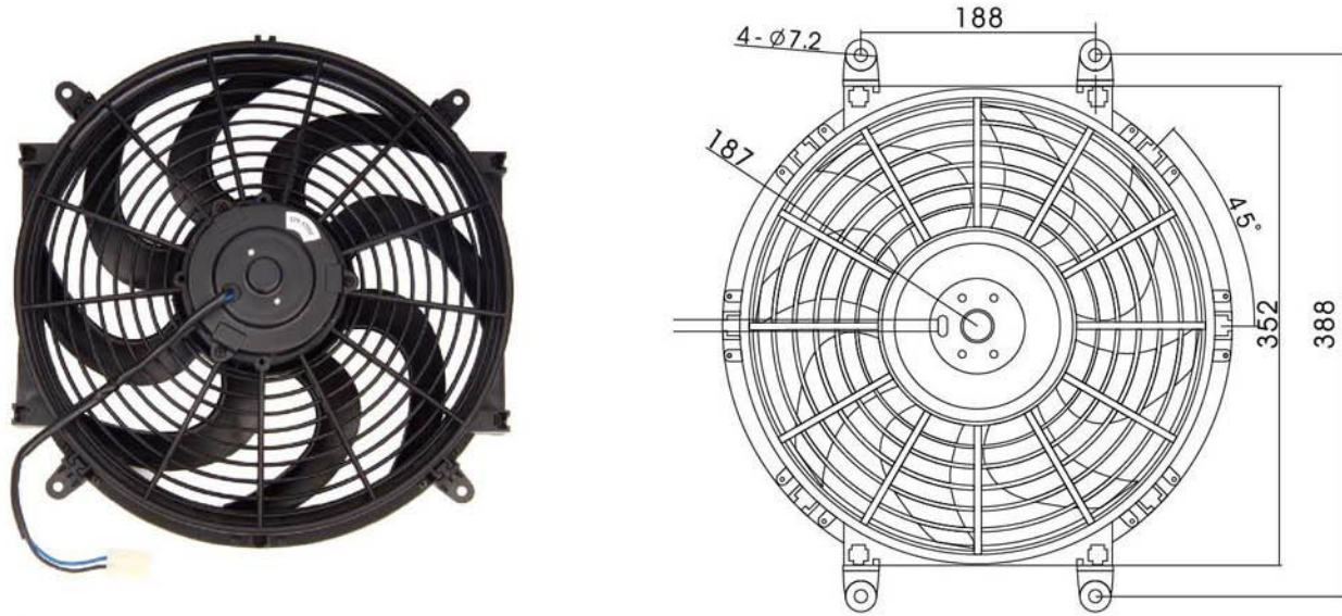
型号: (MODEL):SN81050-14S(90W)
