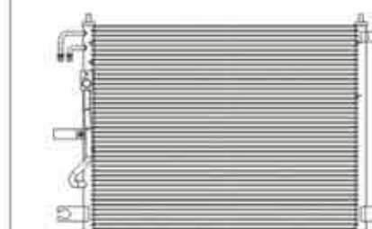
CX-1239 CAR TYPE:AVEO 04-08 CORE SIZE:588X421X18 DPI:3240 OEM:96834083
