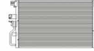
CX-1084 CAR TYPE:EQUINOX 05 CORE SIZE:707X425X20 DPI:3245 OEM:15232871
