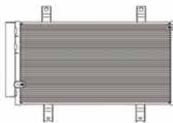
CX-1088 CAR TYPE: MAZDA RX-8 04-10 CORE SIZE: 605X313.4X16 DPI: 3384 OEM: F15161480
