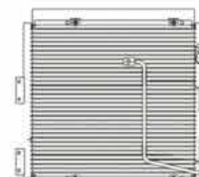
CX-1953AY-16 CAR TYPE:IRAN NPR NOR CORE SIZE:412X369X16 DPI: OEM:
