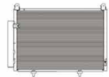
CX-1733 CAR TYPE: Granmax 09- CORE SIZE: 596X391X20 DPI: OEM: 88460-BZ130
