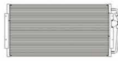
CX-1297 CAR TYPE:LACROSSE CORE SIZE:802X401X18 DPI: OEM:
