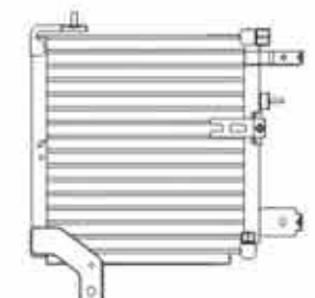
CX-3058 CAR TYPE: Daihatsu Coure CORE SIZE: 329X336.7X32 DPI: OEM:
