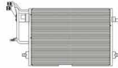
CX-1049 CAR TYPE: AUDI A6 95-04 CORE SIZE: 615X421X16 DPI: 4972 OEM#: 4B0260403T
