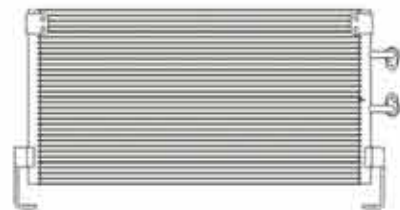
CX-1010 CAR TYPE:DODGE 00-03 CORE SIZE:630X321X18 DPI:4969 OEM:5014582AA
