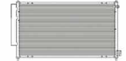
CX-1496 CAR TYPE: AC T.S.X 04-08 CORE SIZE: 696X381X16 DPI: 3295 OEM: 80110SEA013
