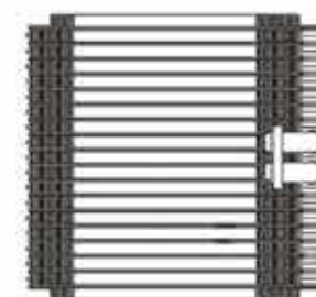
6G-07 CAR TYPE: COROLLA-93 CORE SIZE: 235X85X224 OEM: 8850112370
