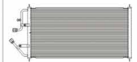
CX-1240 CAR TYPE:C1500 C2500 C3500 CORE SIZE:761X371X20 DPI:4544 OEM:52458718
