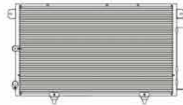
CX-1740 CAR TYPE: LEXUS RX300 99-01 CORE SIZE: 732X419X16 DPI: OEM:
