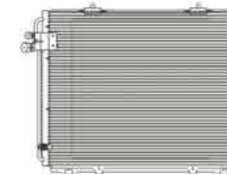
CX-1070A CAR TYPE:08-09 ST A-STRA AT CORE SIZE:586X381X16 DPI:3749 OEM:93178958
