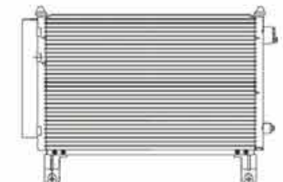
CX-1753 CAR TYPE: DAEWOO CORE SIZE: 534X331.5X16 DPI: OEM:
