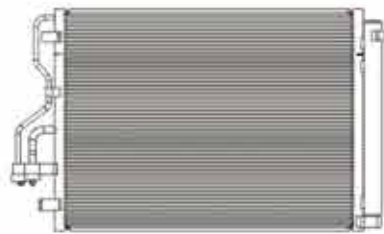
CX-1869Z CAR TYPE:TUCSON 13- CORE SIZE:539X388.2X16 DPI: OEM:97606-2S000
