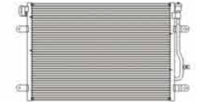
CX-1527 CAR TYPE: AUDI A4 S4 05-08 CORE SIZE: 610X401X16 DPI: 3571 OEM: 8E0260403T
