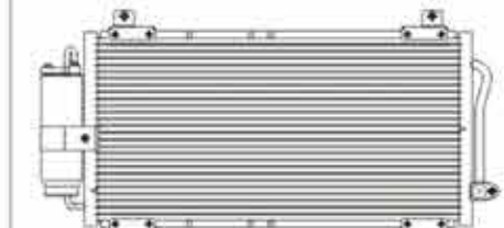
CX-1252 CAR TYPE:CORSA 99/03 CORE SIZE:566X532X16 DPI: OEM:
