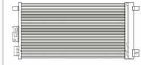
CX-1085 CAR TYPE:04-10 CHEVROLET MALIBU CORE SIZE:698X351X16 DPI:3279 OEM:15777890
