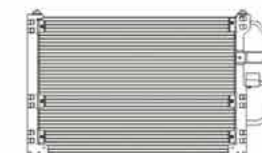
CX-1732 CAR TYPE: LANOS 98-00 CORE SIZE: 595X341X20 DPI: OEM:
