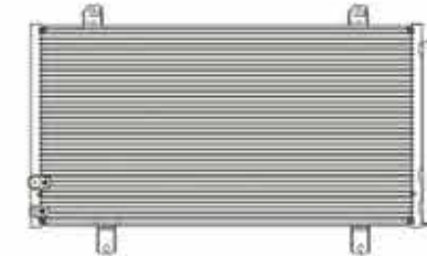
CX-1952ZY-16 CAR TYPE: CAMRY 2013- CORE SIZE: 741X380X16 DPI: OEM:
