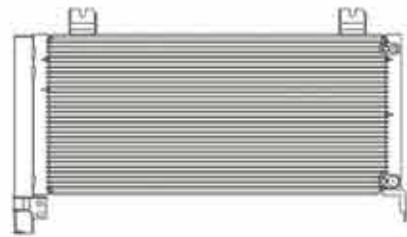
CX-1881H-26 CAR TYPE: LEXUS RX270/350/450 09- CORE SIZE: 735X320X26 DPI: OEM: 88460-48150
