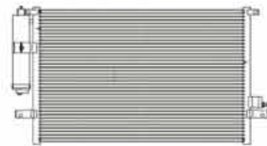
CX-1238 CAR TYPE:BUICK ASTRO CORE SIZE:644X391X18 DPI: OEM:96484931
