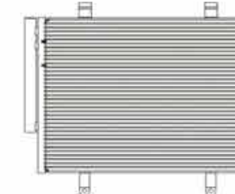
CX-1860 CAR TYPE:SUZUI ERTIGA CORE SIZE:553X388X16 DPI: OEM:
