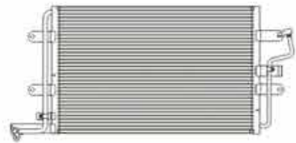
CX-1029 CAR TYPE: AUDI/Skoda Octavia CORE SIZE: 588X361X18 DPI: 4933 OEM#: 1J0820413D
