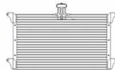
CX-3139 CAR TYPE:Scania New 124 CORE SIZE:818X463.5X22 DPI: OEM:
