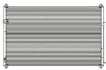
CX-1257 CAR TYPE: MAZDA CX-9 CORE SIZE: 784X461X16 DPI: OEM:
